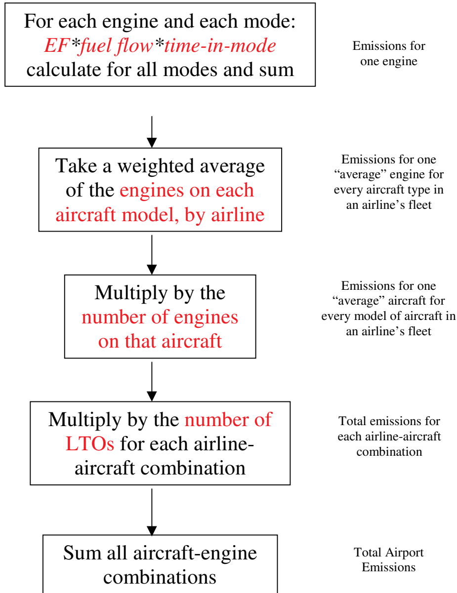
Figure II-3: Aircraft Emissions Calculation Flowchart
