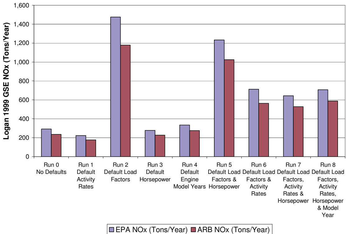
Figure II-6: Logan GSE NOx Emission Sensitivity Analysis Results
